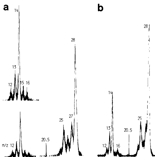
Figure 1. (a) CAMS of ethynamine (m/z 41) produced by FVP of 7b at 740 °C. Inset: higher resolution scan of m/z 12–16. (b) CAMS of m/z 41 (HC≡CNH 2 ++ ) produced by dissociation of HC≡CCONH 2 ++ in the B/E mass spectrometer (see the Experimental Section). The spectra in (a) and (b) were recorded on slightly different scales.
